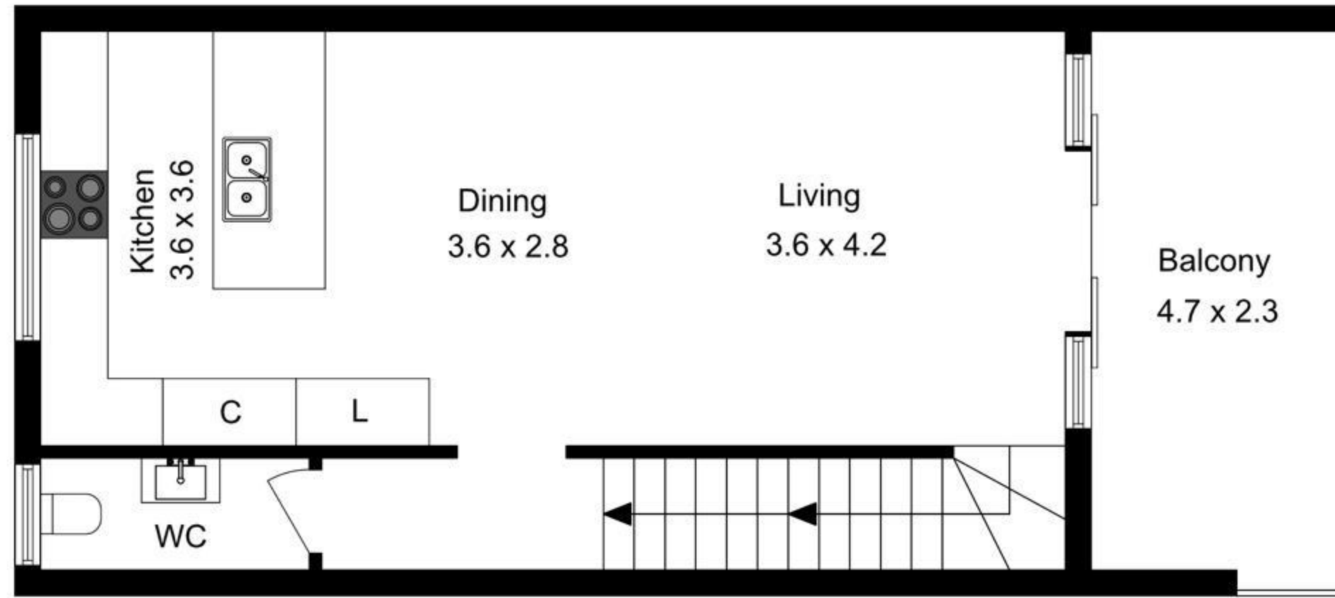
1st Floor
