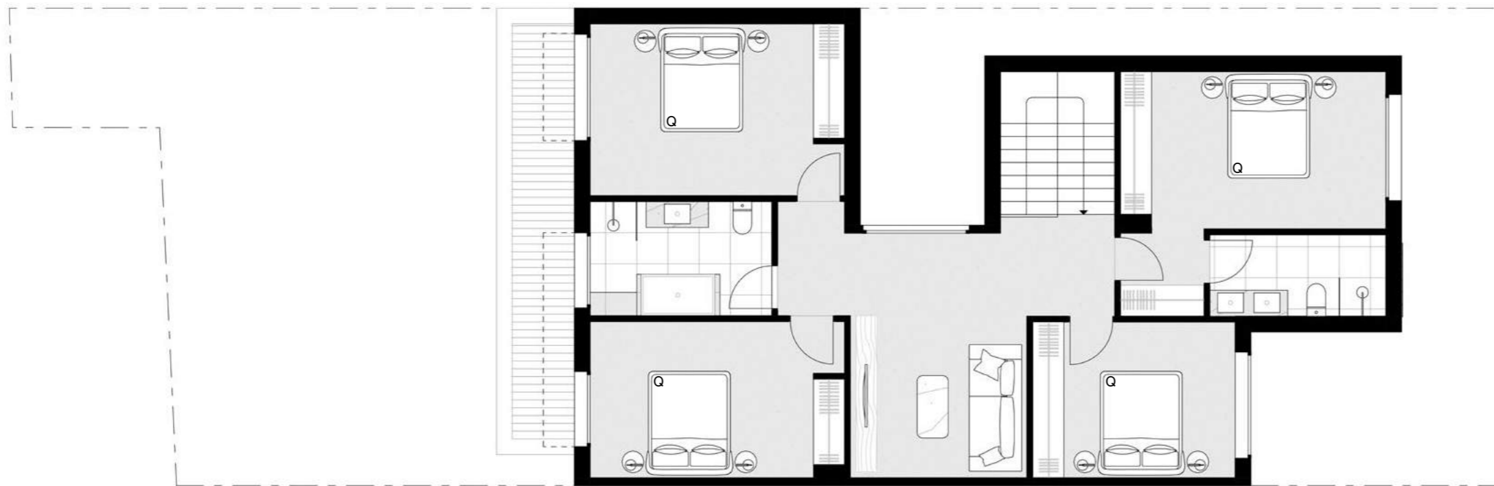
FIRST FLOOR
