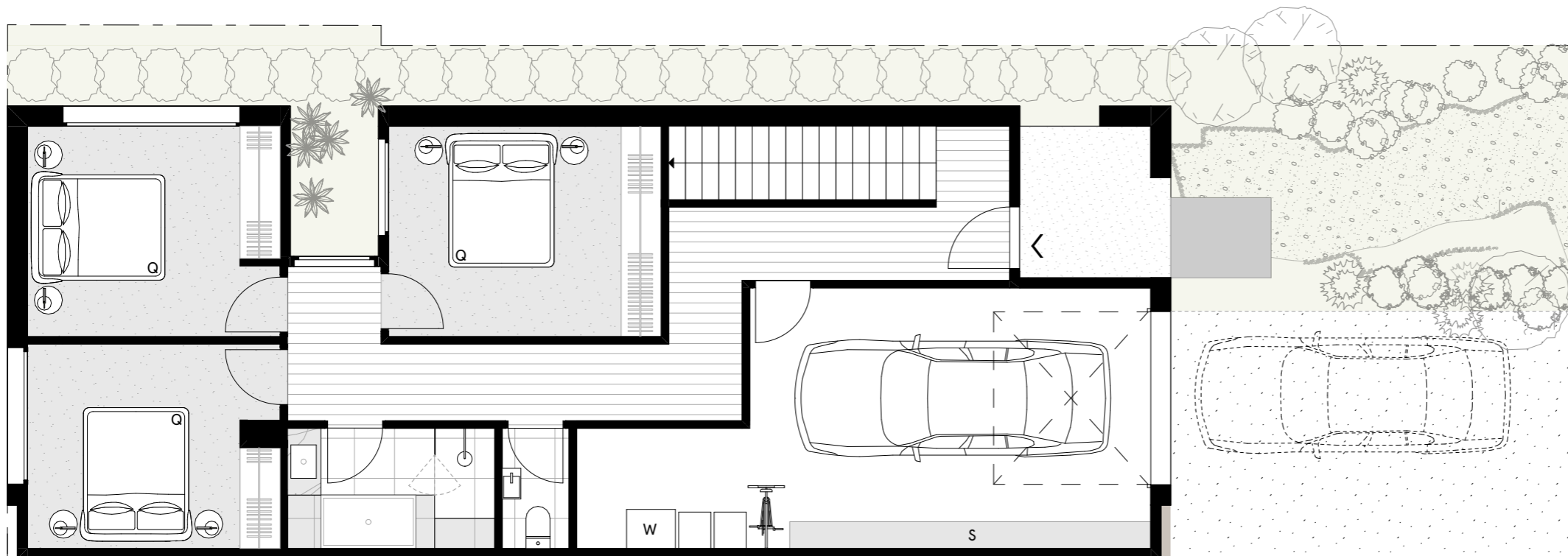
GROUND FLOOR
